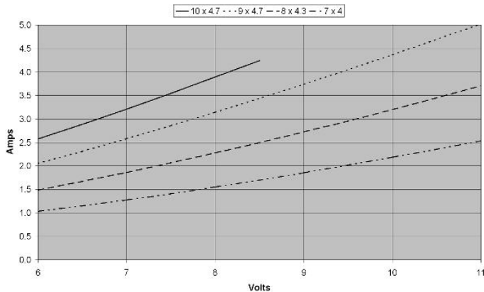
C 2212-0840 - current / voltage with different propellers
