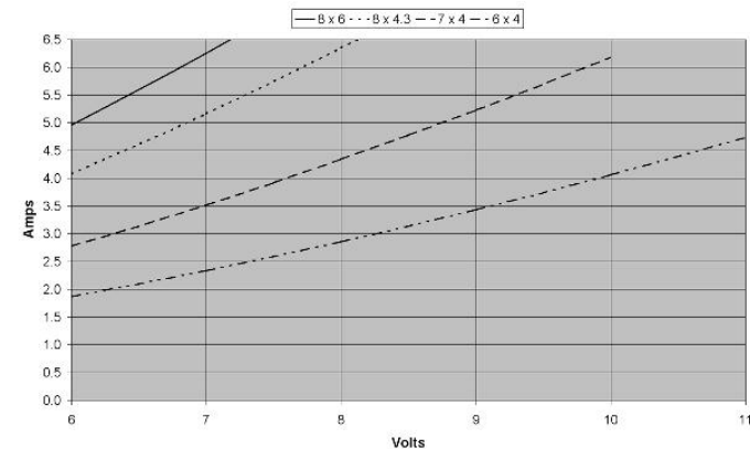
C 2212-1180 - current / voltage with different propellers
