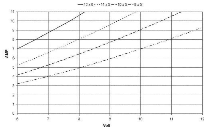
C 2808-0860 - current / voltage with different propellers
