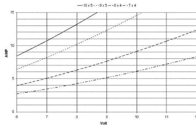
C 2808-1160 - current / voltage with different propellers
