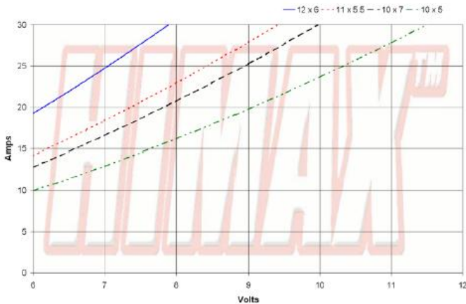
C 3510-1100 - current / voltage with different propellers
