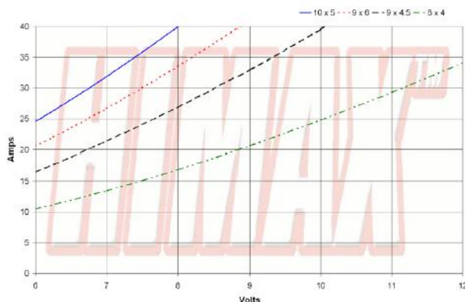
C 3510-1540 - current / voltage with different propellers
