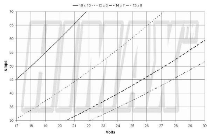
C 5030-0390 - current / voltage with different propellers
