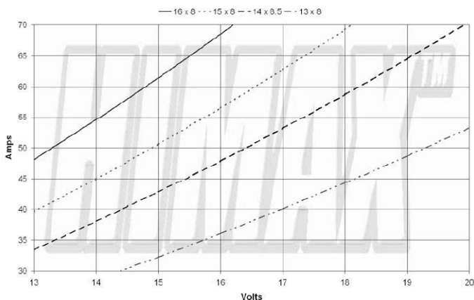
C 5018-0530 - current / voltage with different propellers
