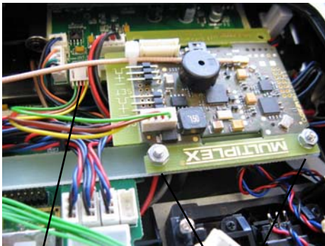
Connector "INT PPM" Washer and Nut M3
