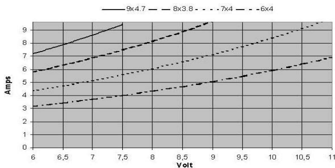
C 2805-1430 - current / voltage with different propellers
