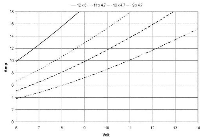
C 2816-0890 - current / voltage with different propellers
