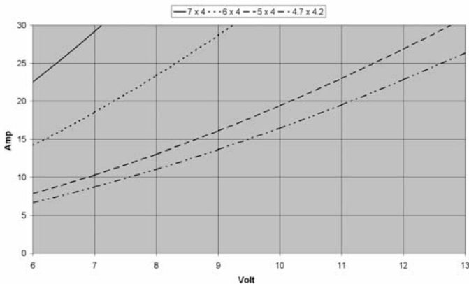
A 2825-2700 - current / voltage with different propellers
