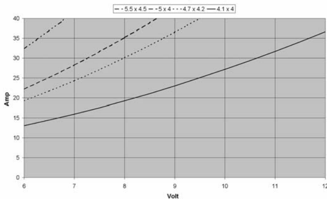
A 2825-3600 - current / voltage with different propellers
