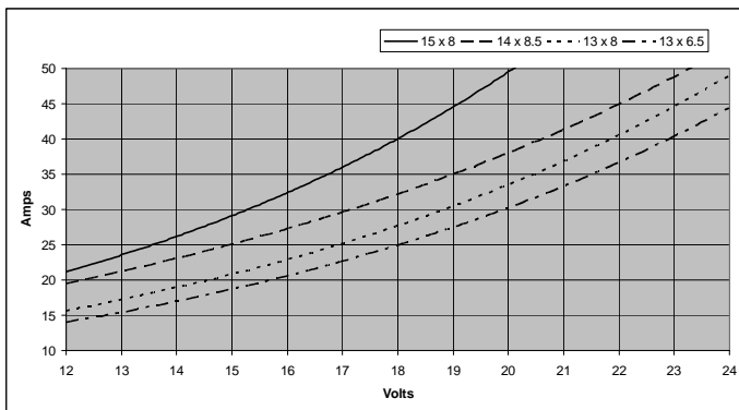
C 4220-0510 - current / voltage with different propellers
