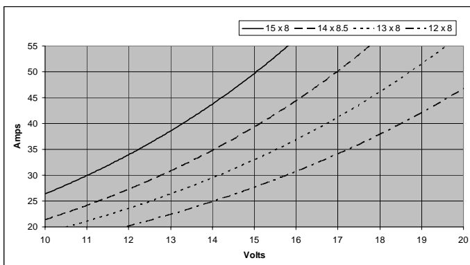
C 4220-0620 - current / voltage with different propellers
